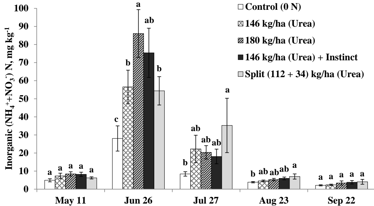
Figure 2: Effect of fertilizer N managements on total soil inorganic ( \text{NH}_4^+ + \text{NO}_3^- ) N, \text{mg kg}^{-1} within 0-30 cm depth under sugarbeet. Bars represent standard errors ( n=8 ). Different lowercase letters within a sampling date are different at 0.05 significance level.
