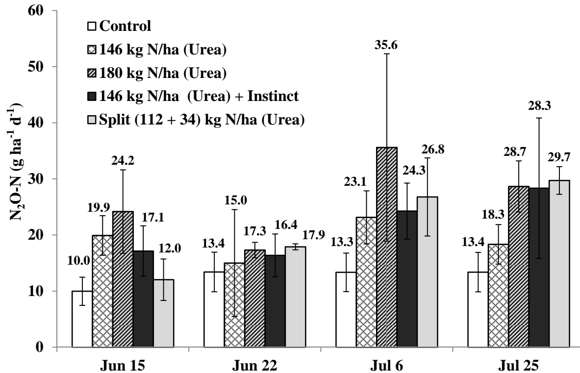
Figure 3. Soil N_2O fluxes after the application of different nitrogenous fertilizer treatments under sugarbeet. Bars indicate standard errors ( n = 4 ).
