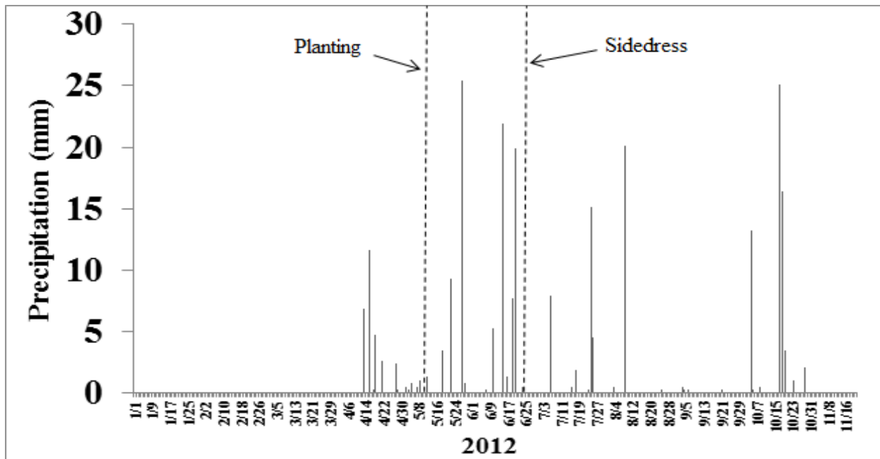
Figure 1. Daily precipitation events in sugarbeet growing season at NW22, near Fargo, ND. The dash lines correspond to the dates for the N fertilizer applications (planting and sidedress).
